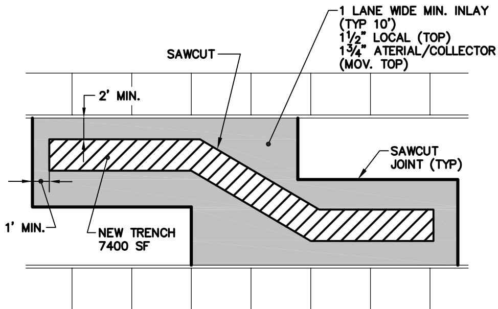
TRENCH ON STREET (>60 MONTHS OLD) NOT TO SCALE
