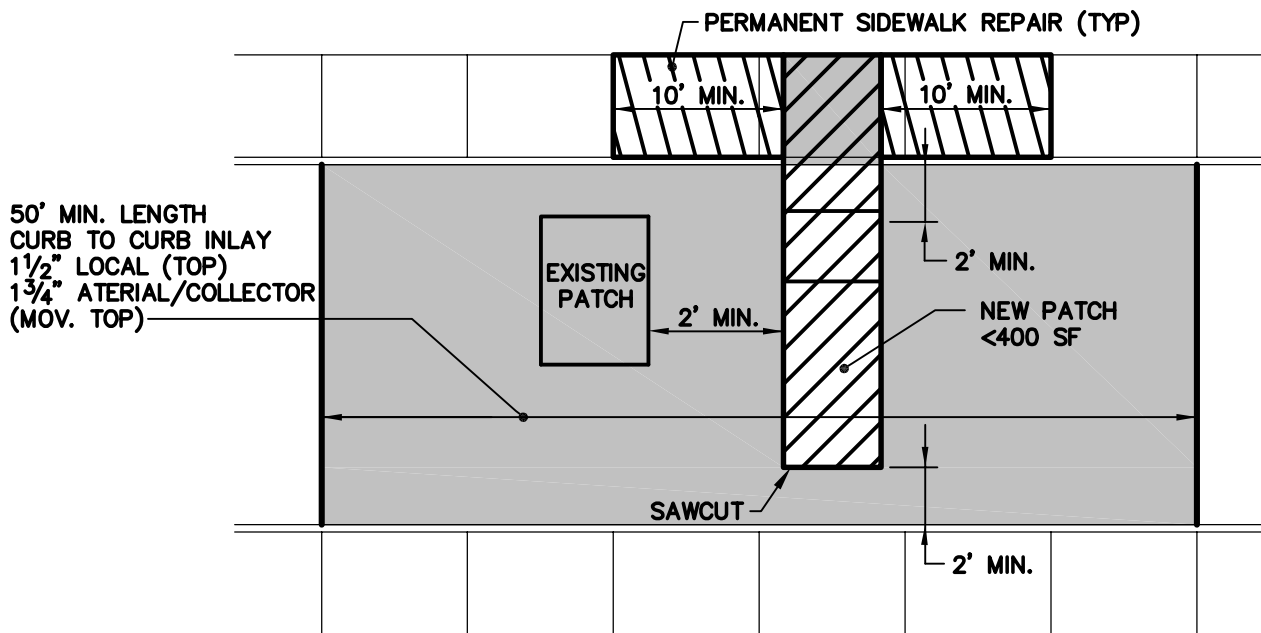
PATCH ON PROTECTED STREET <60 MONTHS OLD) NOT TO SCALE
